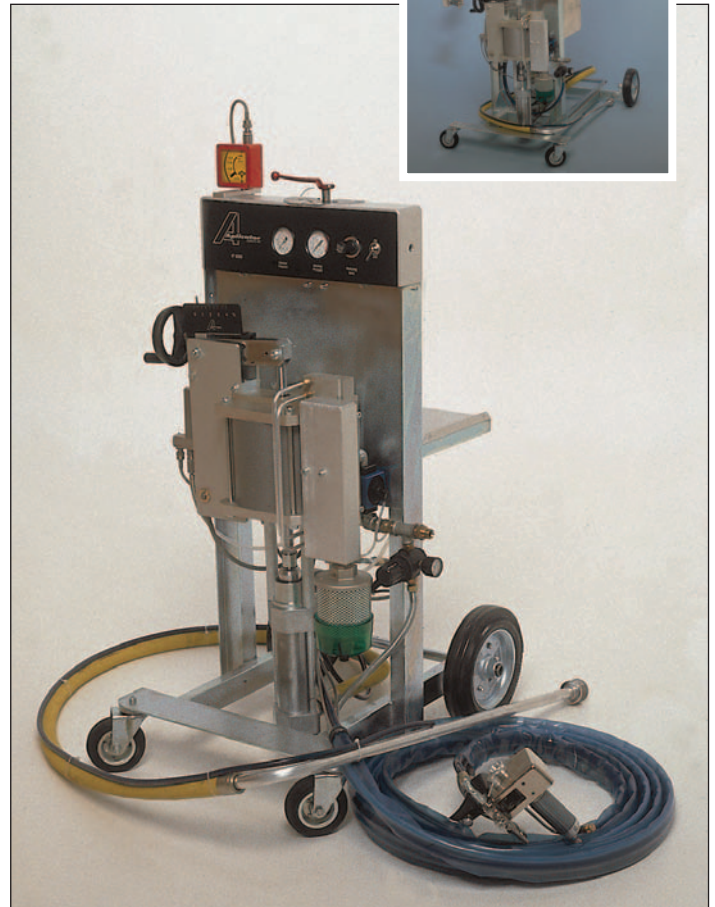
IPS-8000 equipped with drum cart and boom
